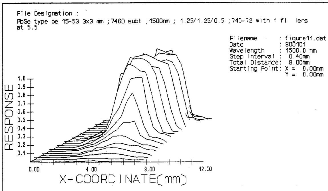
Figure 11 - PbSe DETECTOR UNIFORMITY PROFILE AT 1.5 MICRONS.
